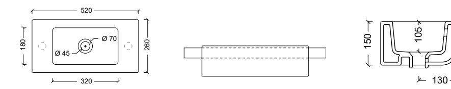
20170501 Lavabo ICE 52 X 26
