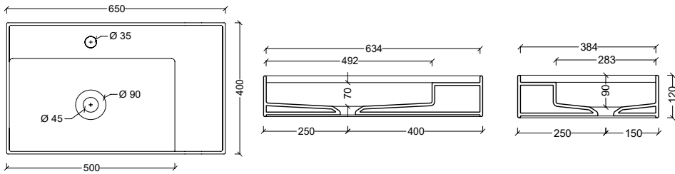
31120101 Lavabo HIDE STADIUM
