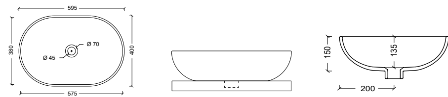
29170101 Lavabo JOKER POT
