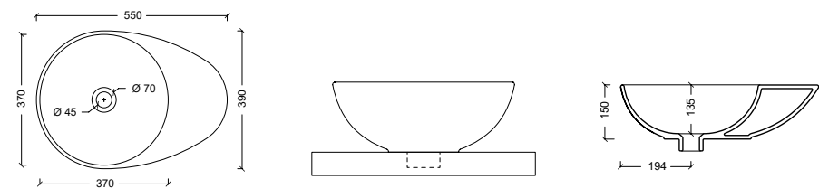
29150101 Lavabo JOKER EGG
