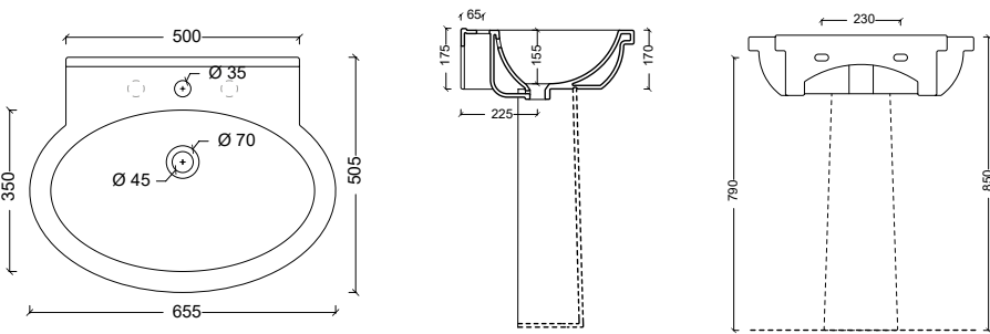
30200101 LAVABO SHORT 65
