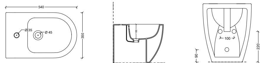
22270101 Vaso a terra H 50 FORM SQUARE RIMLESS
