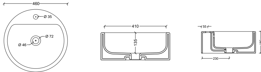
22100301 Lavabo FORM 46 ROUND
