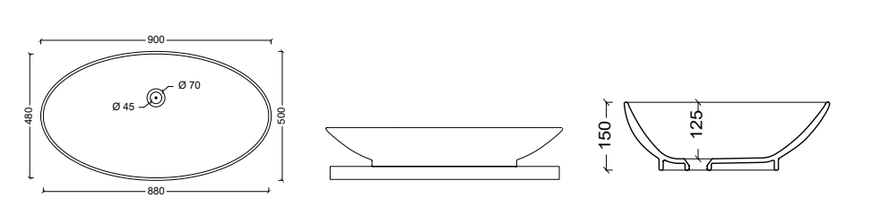
29210301 Lavabo JOKER DISH
