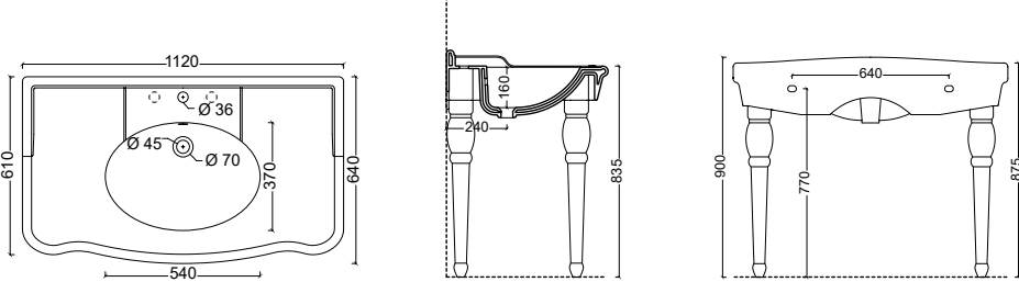
28250101 Console BOHEME 112
