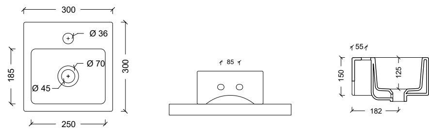
20140101 Lavabo ICE 50 X 27
