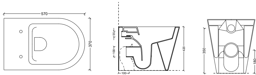
31150101 Vaso a terra HIDE ROUND
