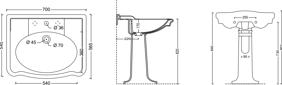
28230101 Lavabo BOHEME 70
