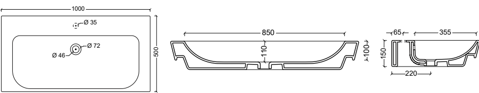
22160101 Lavabo FORM 100
