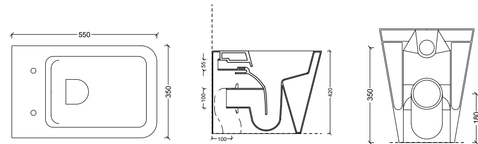
31190101 Vaso a terra HIDE SQUARE
