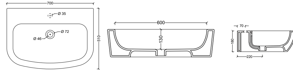
22140101 Lavabo FORM 70
