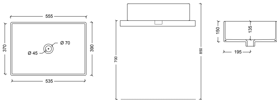
29120101 Lavabo JOKER CHEESE
