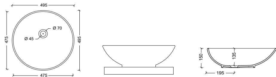
29160101 Lavabo JOKER BOWL
