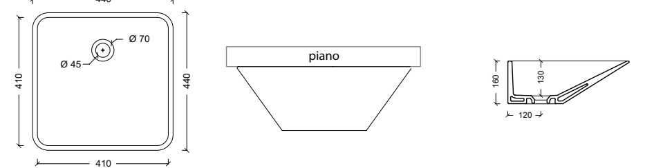
26110401 Lavabo EDGE 44X44 UNDERCOUNTER
