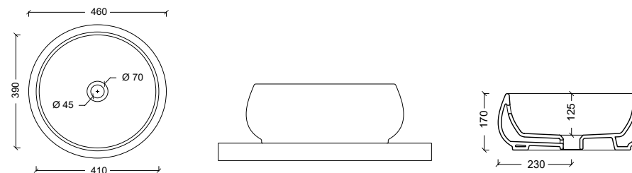
24100301 Lavabo TULIP SMALL
