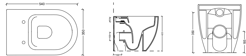
22250101 Bidet a terra FORM SQUARE
