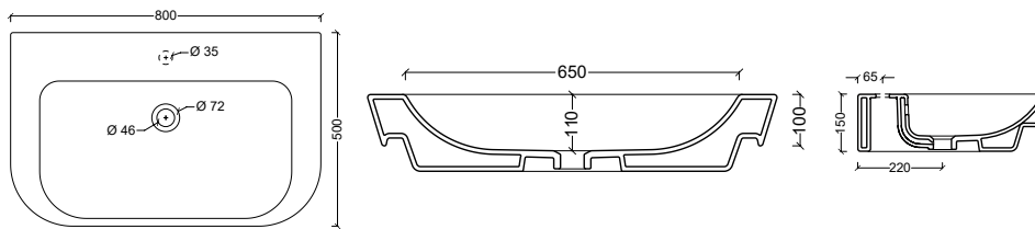
22150101 Lavabo FORM 80
