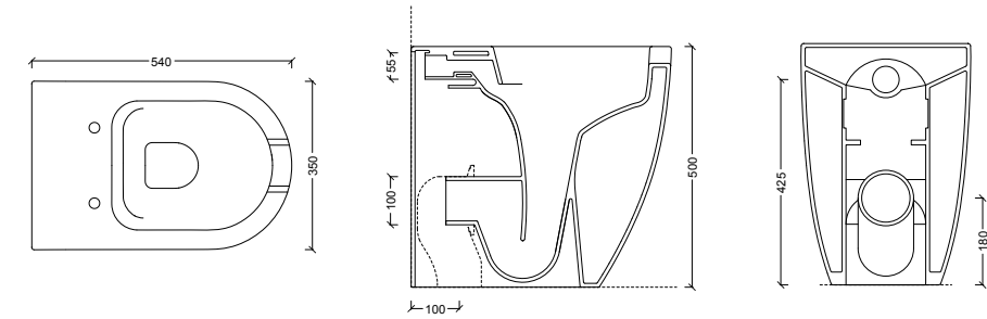
22320101 Vaso a terra H 50 FORM SQUARE OPEN
