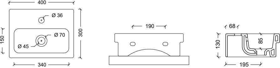
21160801 Lavabo LOGIC 35 X 35
