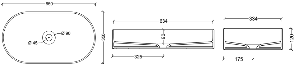
31120101 Lavabo HIDE STADIUM
