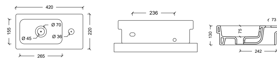
21150801 Lavabo LOGIC 42 X 22
