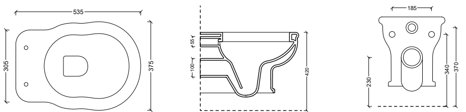
28230101S Vaso sospeso BOHEME
