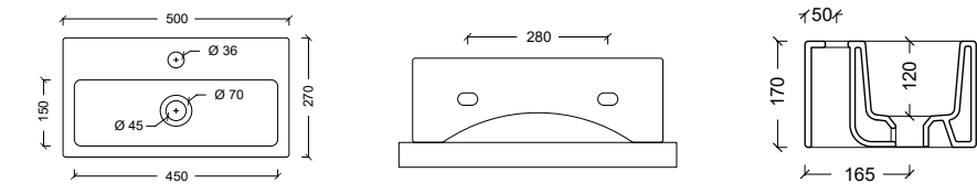
20100101 Lavabo ICE 40 X 20
