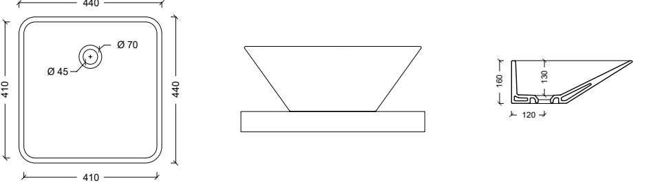
26110401 Lavabo EDGE 44X44 UNDERCOUNTER
