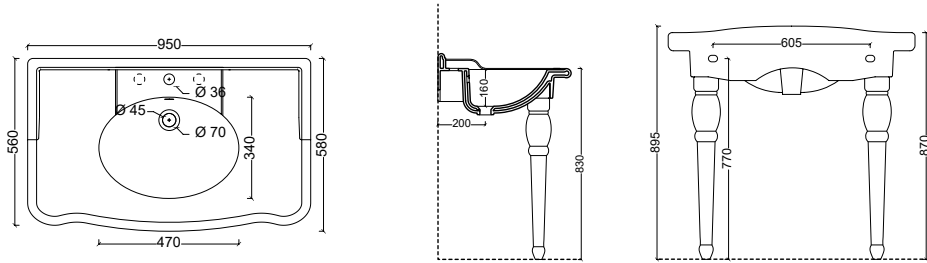
28260101 Lavabo Console BOHEME 95
