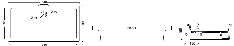
27110401 Lavabo CUBIC 80
