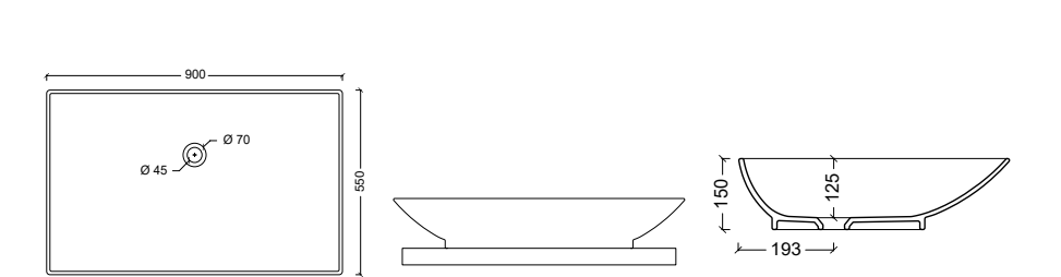
29200301 Lavabo JOKER TRAY
