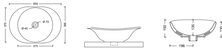
29150101 Lavabo JOKER EGG
