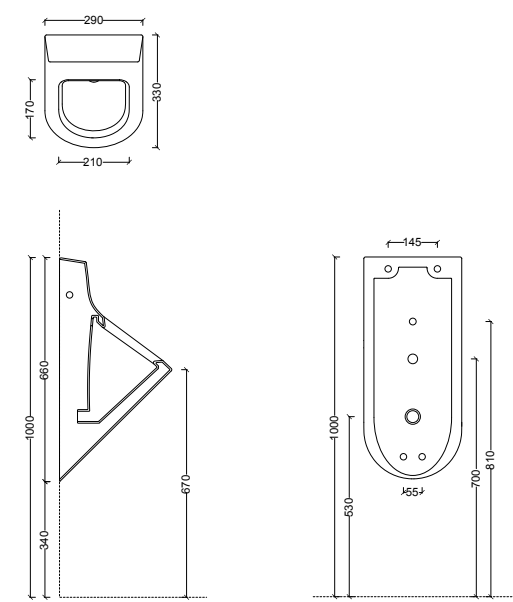
22260101 Orinatoio FORM
