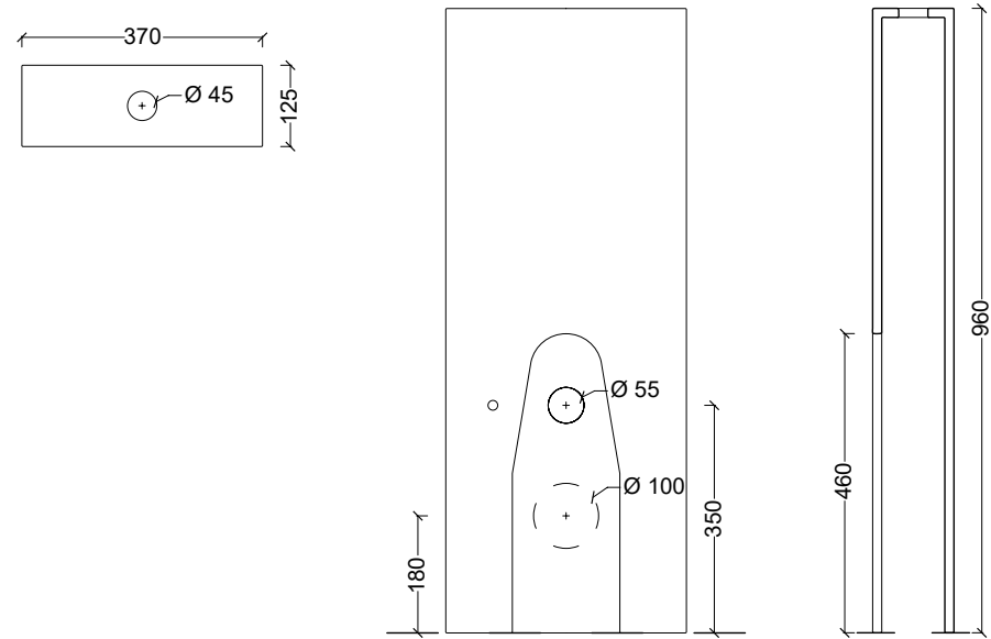
26900101 HIDE Cistern
