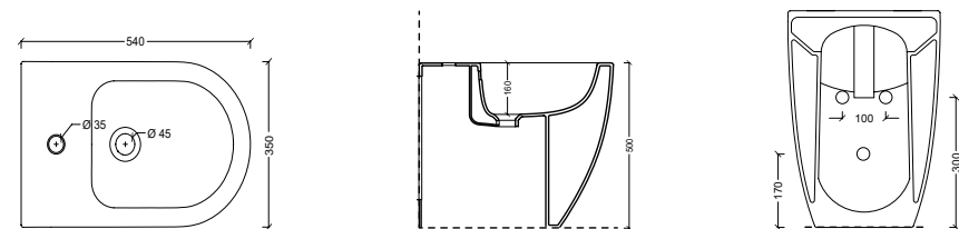
22280101 Bidet a terra H 50 FORM SQUARE
