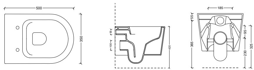
22300101RL Vaso sospeso FORM SQUARE
