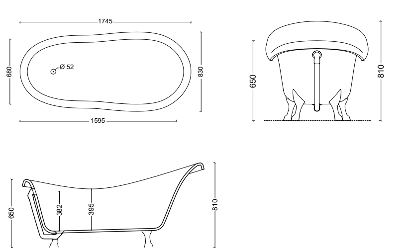
VABO Vasca BOHEME
