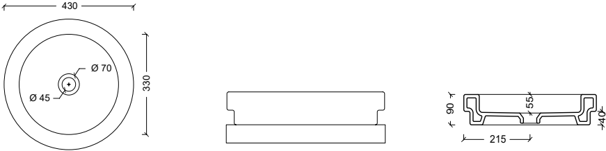
21140701 Lavabo LOGIC 43
