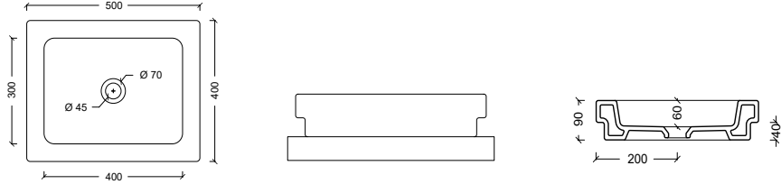
21140701 Lavabo LOGIC 43
