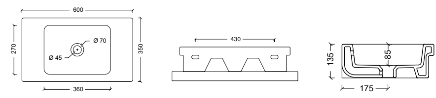
21120801 Lavabo LOGIC 45 X 30
