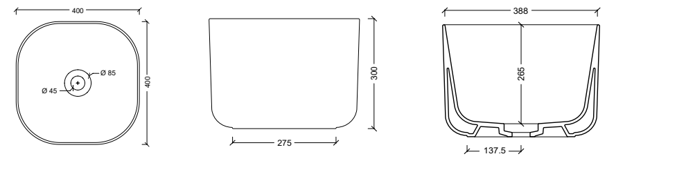
32150101 Lavabo UNICA RECTANGULAR
