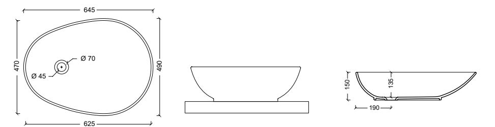
29130301 Lavabo JOKER SPOON
