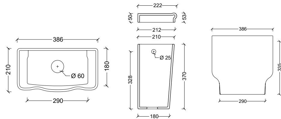
28320101 cassetta alta BOHEME
