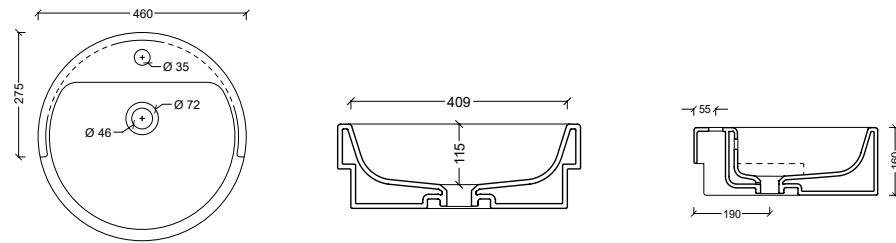
22100301 Lavabo FORM 46 ROUND
