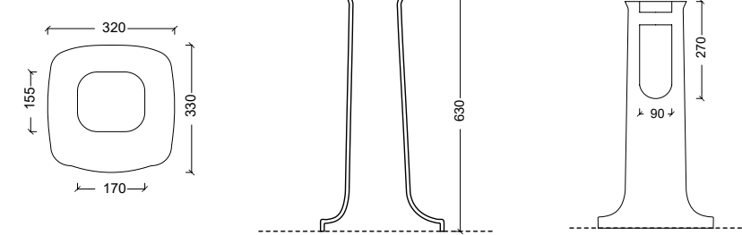
28240101 Colonna LAVABO BOHEME 70
