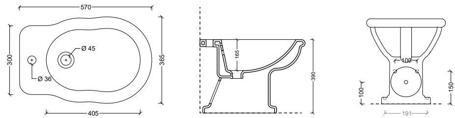
28220101 Bidet a terra BOHEME
